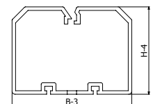
RCQRL H80/H100/H120
